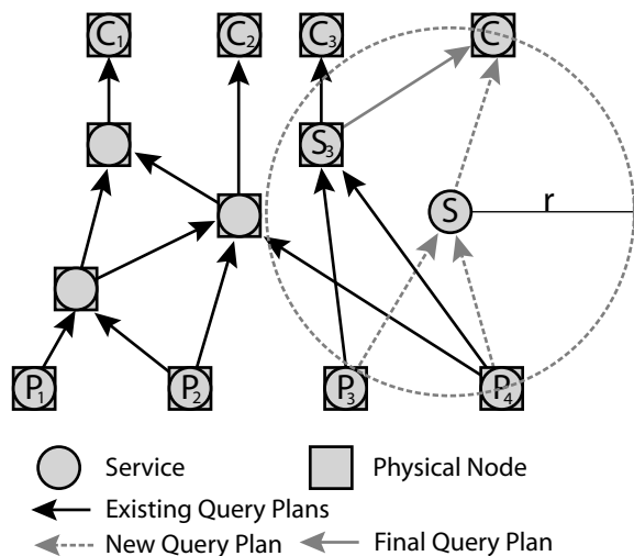
Fig. 4. Example of multi-query optimization in a cost space. The example shows a multi-query optimizer only considering services within a radius r of a new service S in a 2-dimensional latency cost space.
