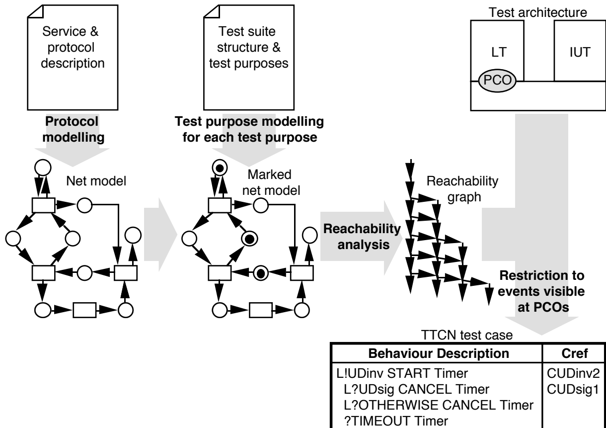
Figure 2 Test case generation from net models
