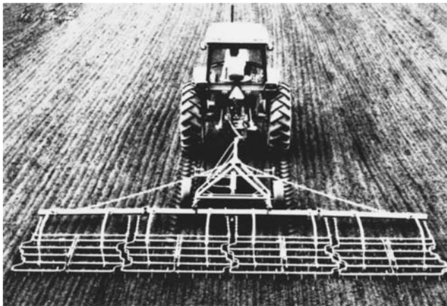
Figure 44 – Harrow—Four sections, spike teeth—Squadron hitch
