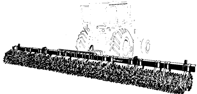
Figure 47 – Rotary hoe—In-line sections on spring loaded arms—Rear-mounted
