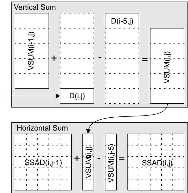
Figure 7: SSAD computation 2
