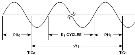
Figure 5. Carrier phase counting.
