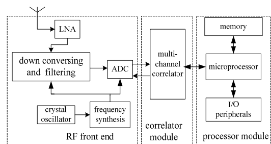
Figure 1. The whole framework of GPS receiver.
