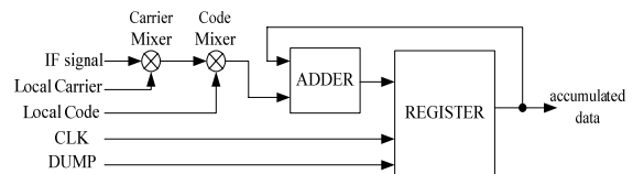
Figure 7. The construction of Correlating Accumulator. 95
