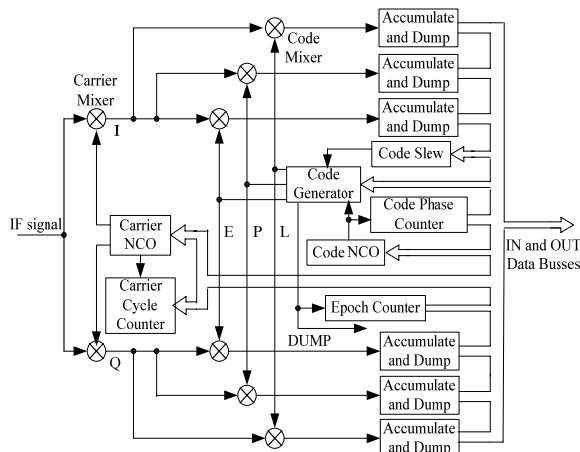
94 Figure 3. The construction of Tracking Channel.
