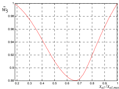
Figure 5. Manipulability of the mobile manipulator
