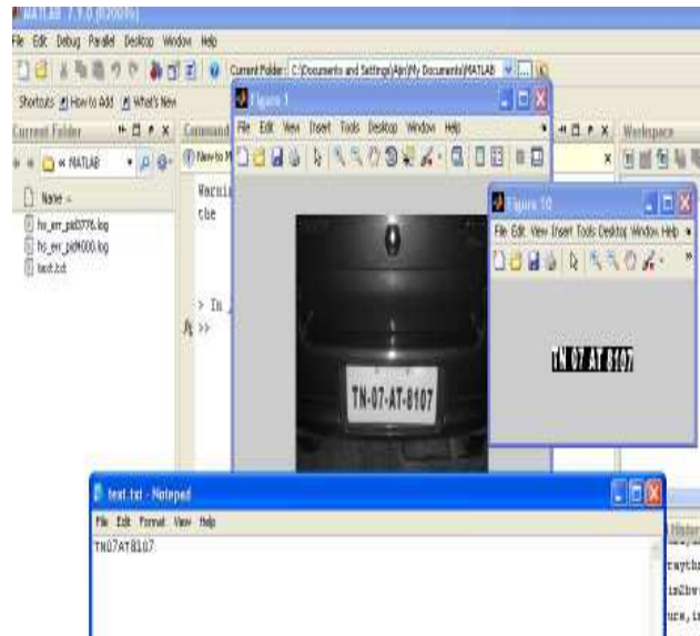
Fig. 9: Snapshot of the notepad displaying the recognized characters
