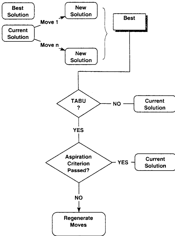
Fig. 10. Flowchart of the short-term Tabu search algorithm.
