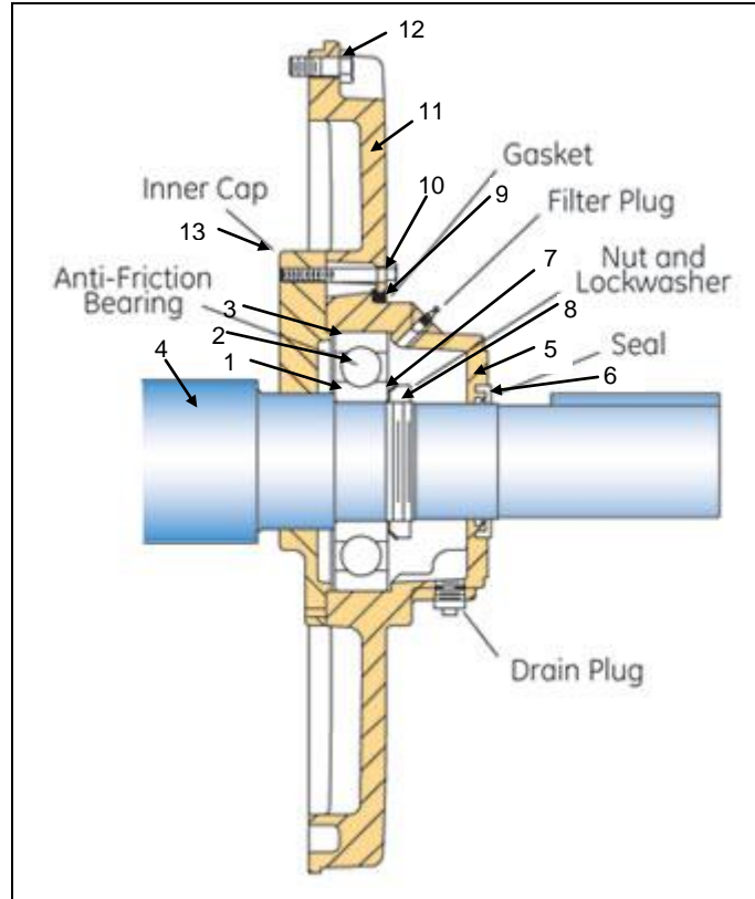
Figure 2 –Series Arrangement of Parts Allow a Shaft to Turn in a Electric Motor Bearing Housing
