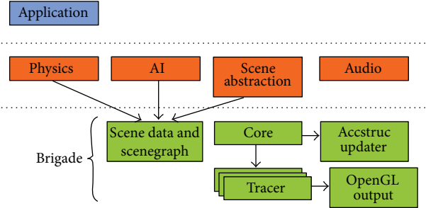
FIGURE 6: Functional overview of the Brigade renderer, combined with a generic game engine.
