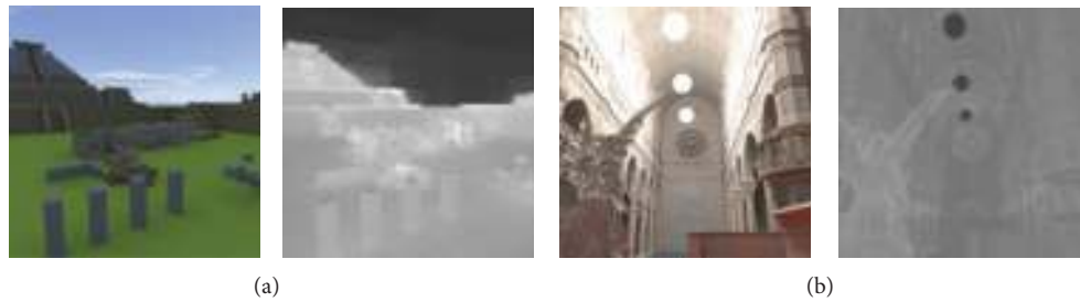
FIGURE 10: Render cost visualized: pixels representing the sky dome or light sources have a significant lower cost than other pixels. Cost is represented by greyscale values (brighter is higher cost), per 32 pixels (a full warp). Measured using a tracer implemented in NVidia’s CUDA [11] for two scenes: Aztec (a) and Sibenik Cathedral (b).
