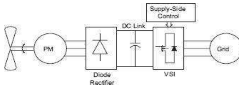
Fig.3 Hard Switching Supply side Inverter with Voltage Source Inverter (VSI)
