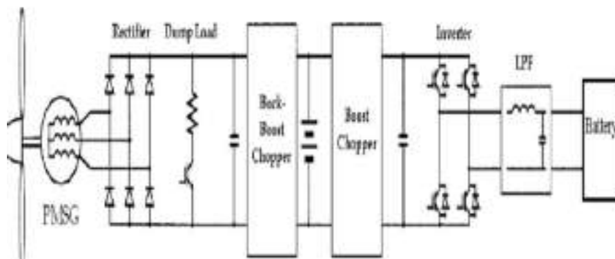
Fig. 12 DC boost & DC buck-boost with PMSG
