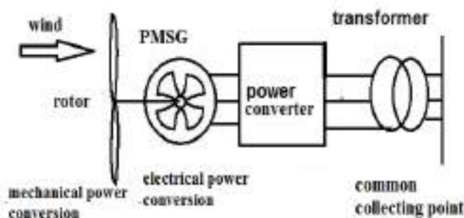
Fig. 1 Wind energy conversion system for PMSG
