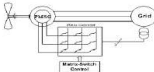
Fig. 6 Conventional matrix converter
