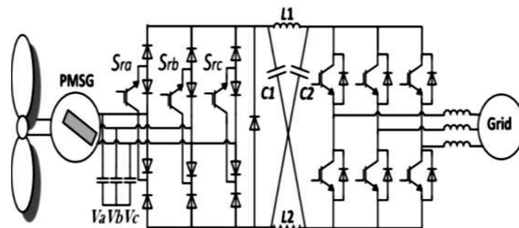
Fig. 11 Z-source inverter
