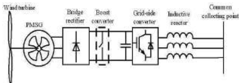
Fig. 5 Generator side uncontrolled rectifier with boost converter
