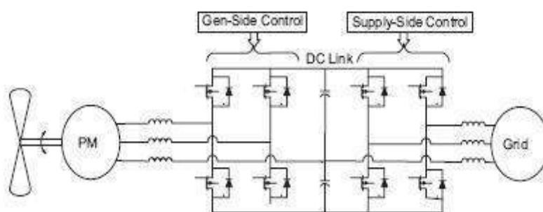
Fig. 4 Back to back PWM VSI converter
