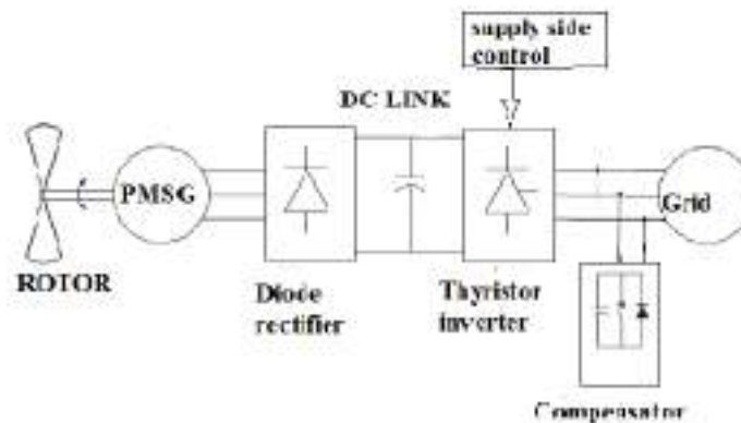
Fig. 2 Thyristor grid side converter
