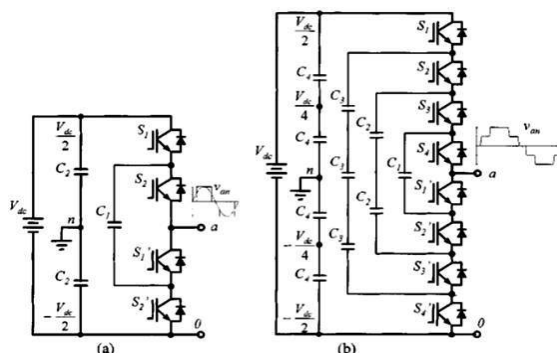
Fig. 9 Flying capacitor converter (a) 3-level (b) 5-level
