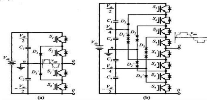
Fig. 8 Neutral clamped or diode clamped converter (a) 3-level (b) 5-level
