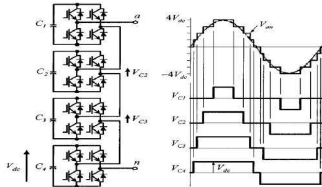
Fig. 10 Clamped capacitor converter
