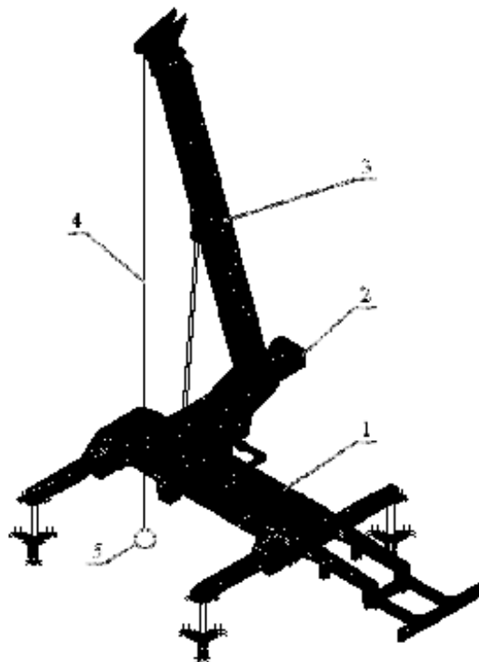
Fig. 1. Model of truck crane (1 - chassis frame, 2 - body frame, 3 - crane boom, 4 - linear system, 5 - mass of load)
