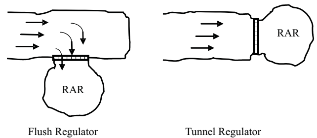
FIG 3 - Graphical examples of flush and tunnel regulator layouts.
