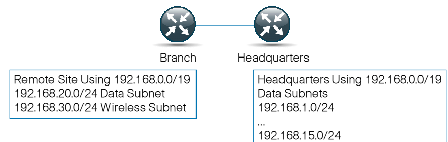
Figure 5. Overlapping IP Address Space, Non Conflicting
