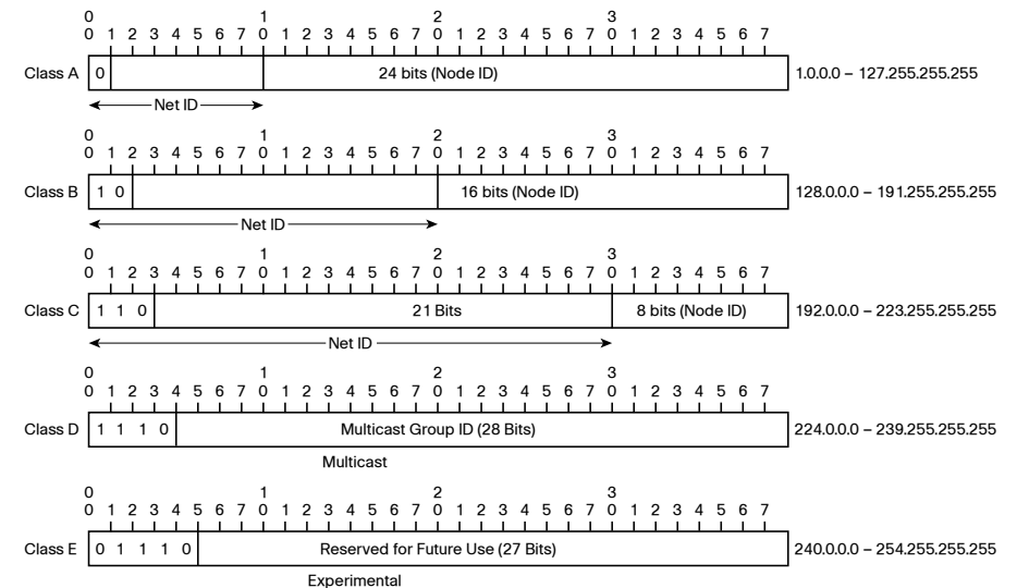
Figure 1. Classful Addresses
