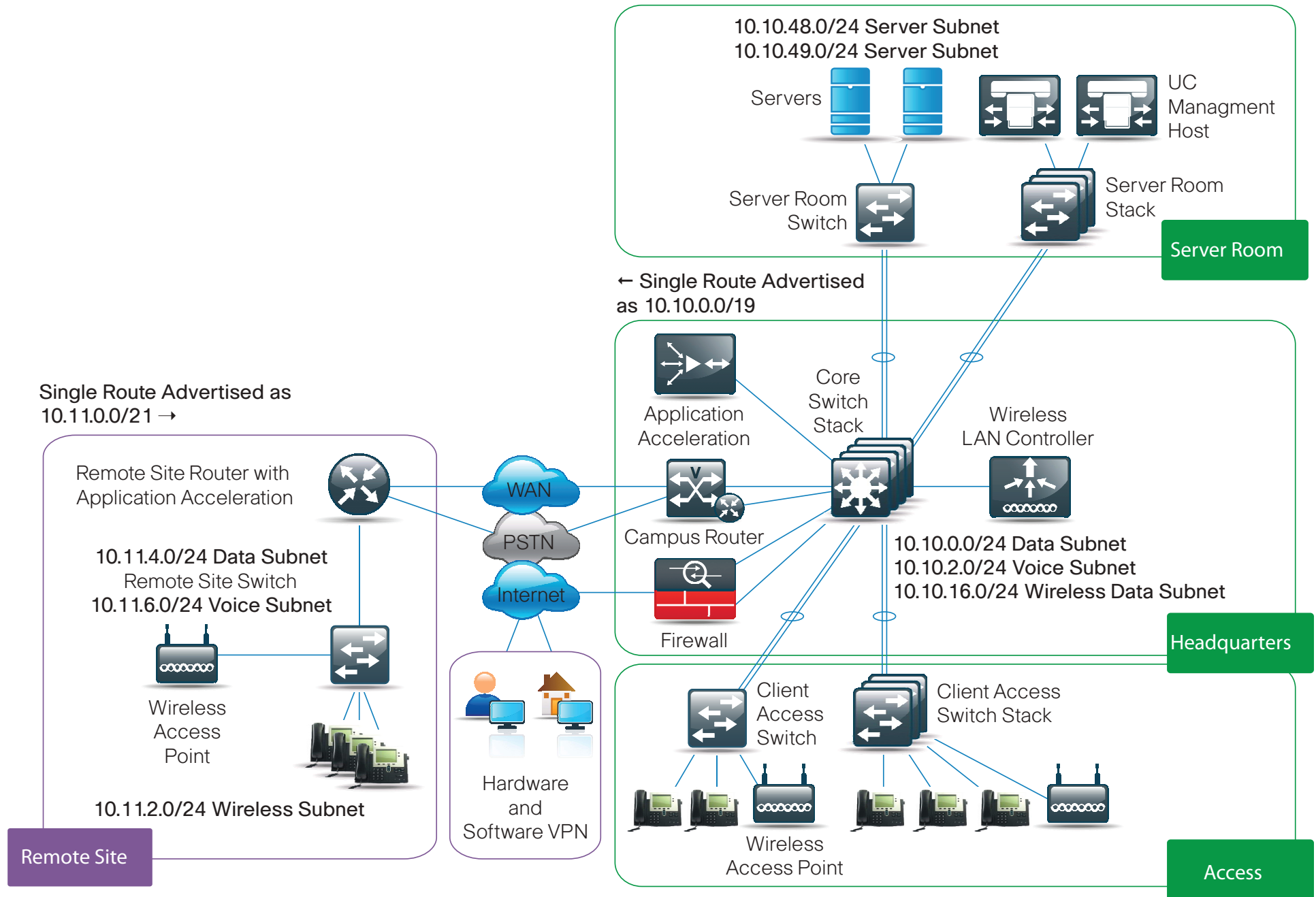
Figure 4. Cisco SBA Design with Assigned IP Addresses and Summarization
