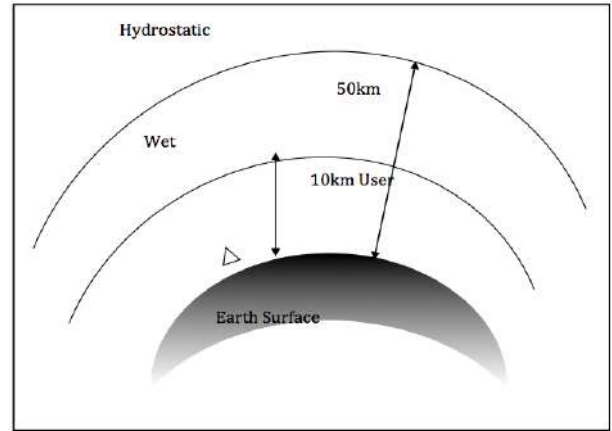
Figure 1. Schematic diagram of the Hydrostatic and Wet components of the troposphere [9]
