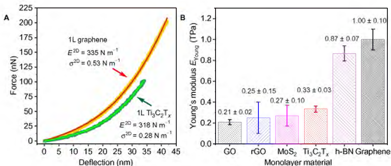
Fig. 3. Comparison of indentation tests on Ti_3C_2T_x with other 2D materials. (A) Comparison of experimental F-\delta curves for monolayer graphene and Ti_3C_2T_x membranes. (B) Comparison of effective Young's moduli for several 2D materials: GO (12), rGO (13), MoS 2 (5), h-BN (8), and graphene (7). In this chart, we compare values produced on membranes of monolayer 2D materials in similar nanoindentation experiments.
