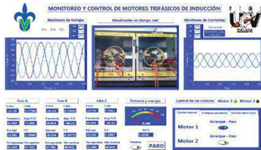
Figure 4. Front panel of the main virtual instrument developed for the control of two AC induction motors [17].
