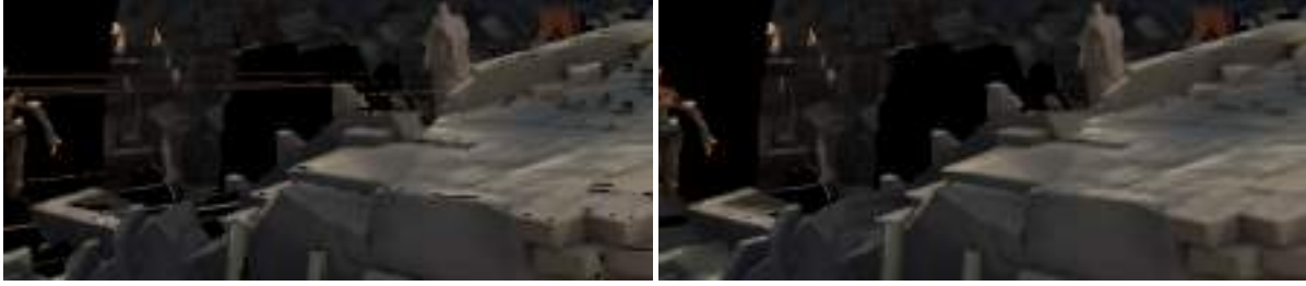
Figure 3: Wrongly connected mesh (left): connections over object boundaries (causes stripes) and missing connections (causes black spots). Our meshing algorithm was able to remove most of these artifacts (right). (detail from the temple2 sequence)
