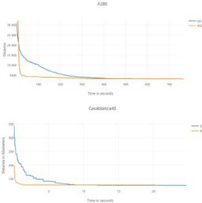
Fig12– Overlaid computational results of GA and ACO
