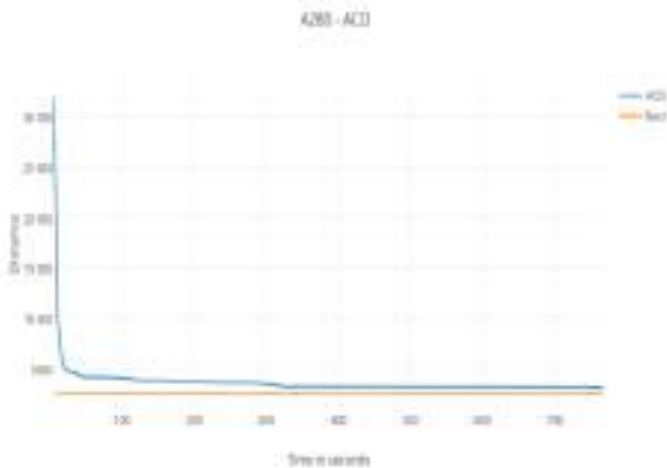
Fig9- Evolution of ACO results over time in A280
