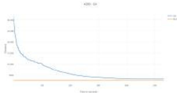
Fig3- Evolution of GA results over time in A280
