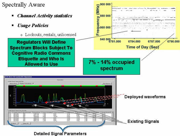
Figure 7 – Spectrum Awareness. A CR or a set of CRs may be aware of the spectrum and may exploit unoccupied spectrum for their own purposes.
