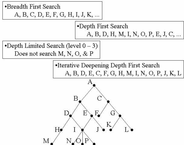
Figure 6 – Search Algorithms. Various state search algorithms yield different performance, time or space complexity, as a function of environment.
