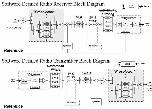
Figure 2 – General SDR RF Frontend. The RF Frontend has the following sections: Pre-selector / Power Amplifier, Receive Chain, Transmit Chain, and Synthesizer [1].
