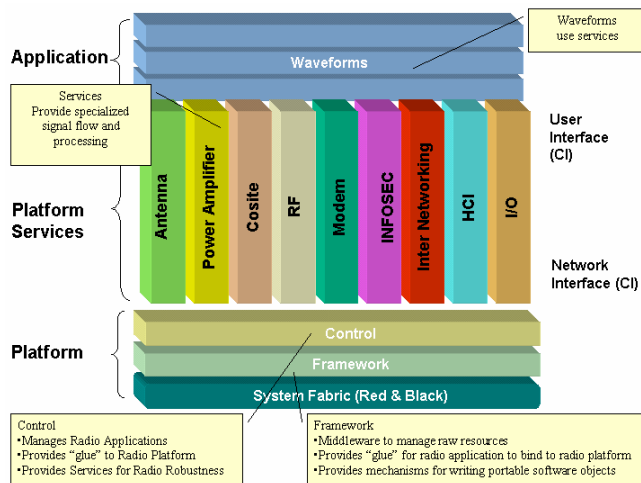
Figure 4 – SDR Software Architecture. A layered SW architecture supports SW portability and enables CR applications to be added easily.
