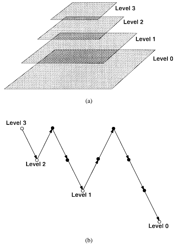
Fig. 1. Multigrid. (a) A four-level multigrid pyramid. (b) A full multigrid V cycle.
