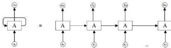
Figure 1. The fragment of recurrent neural network and an unrolled recurrent neural network..
